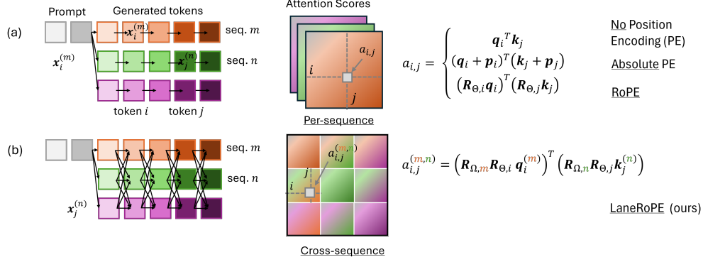
Figure 2: Comparison of RoPE [30] and LaneRoPE for parallel inference. (a) Parallel inference (e.g., best-of-N) relies on generating sequences independently. As a result, positional encodings and attention scores are defined only per-sequence. (b) With LaneRoPE, tokens are generated by causally attending to tokens from all sequences. We achieve this by introducing cross-sequence attention scores with a novel position encoding scheme to account for inter-sequence relative distances.
