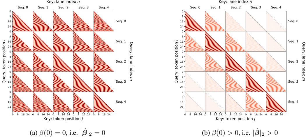
Figure 3: Effect of the attention bias \beta on attention scores in LaneRoPE, controlled by |\hat{\beta}|_2 . A GroupThink initialization is used, where tokens from different lanes occupy distinct virtual position indices. The causal mask within each lane is preserved.
